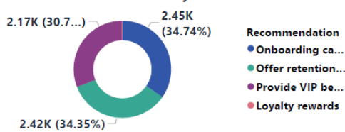
Count of Customers by Recommendation
