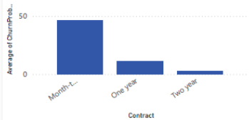
Average of ChurnProbabilityPercent by Contract
