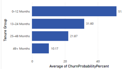
Average of ChurnProbabilityPercent by Tenure Group
