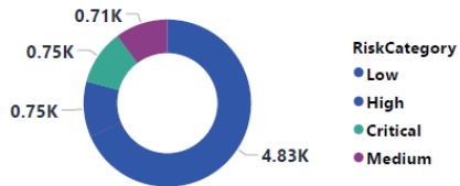
Customer Risk Distribution
