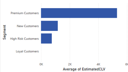
Average of EstimatedCLV by Segment
