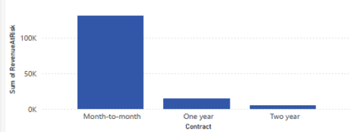
Sum of RevenueAtRisk by Contract
